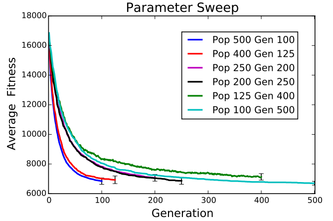
Figure 5. The heuristic is robust with respect to a range of parameter settings.
