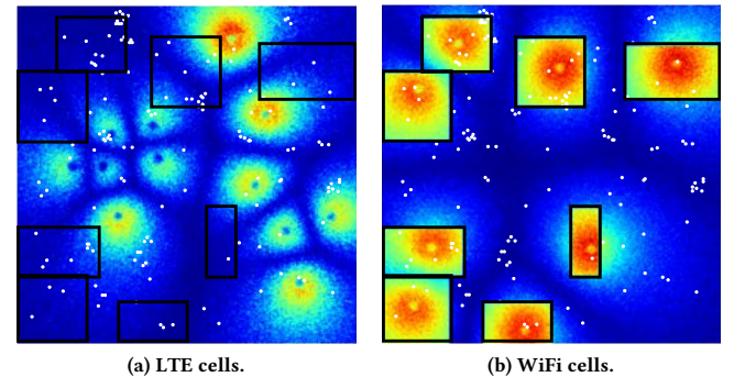
Figure 4: LTE and WiFi cells transmit data to users (white dots) in an enterprise environment. Black lines indicate the exterior walls of buildings. Signal qualities are lowest at cell edges.
