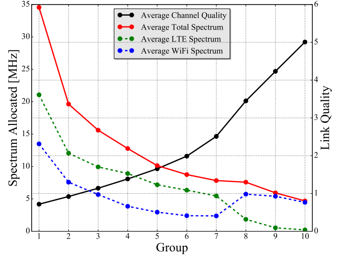
Figure 8: Fairness is achieved by allocating more spectrum to the users with low aggregate link quality. Users in groups 8, 9, and 10 are allocated more WiFi spectrum because they are primarily inside buildings.
