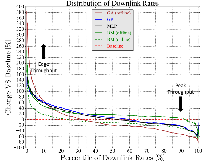
Figure 6: The distribution of downlink rates under various schemes for link allocation are compared relative to a single-link baseline technique. The goal is to increase cell edge throughput versus the baseline. An inherent tradeoff between cell edge and peak throughput is evident.
