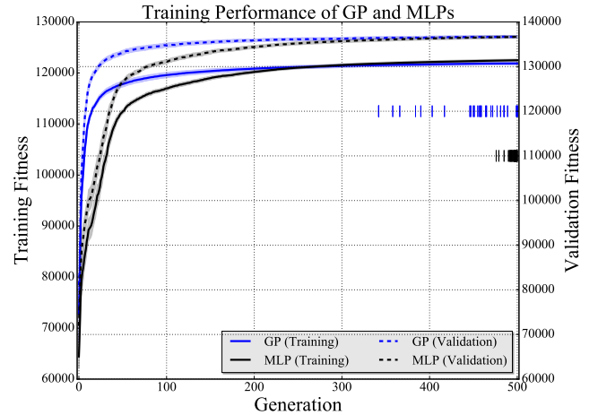
Figure 5: The average training and validation fitness for the 30 GP and MLP runs is plotted over generations. Shaded 95% confidence intervals enclose the average fitness. Vertical strikes indicate when the best scheduler is discovered.
