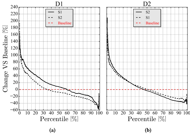
Figure 7: GP generates specialized schedulers that are adapted to their deployment context. Downlink rates are computed for users in 30 time slots.
